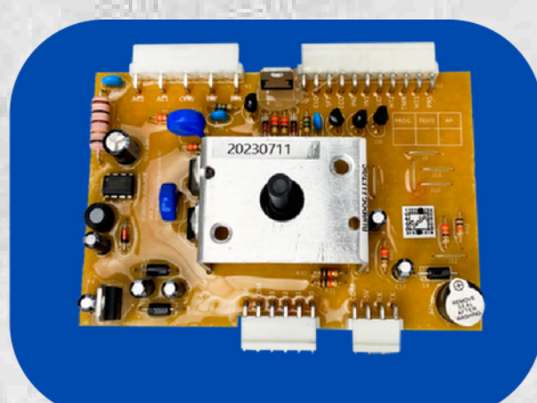
6413 POTENCIA COMPATIVEL LT12B BIVOLT 60HZ A99035178 A99035101
